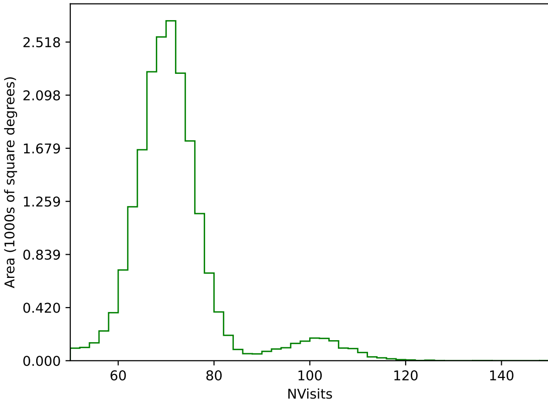
start_date_do-270v3.4_10yrs All sky g band: NVisits
