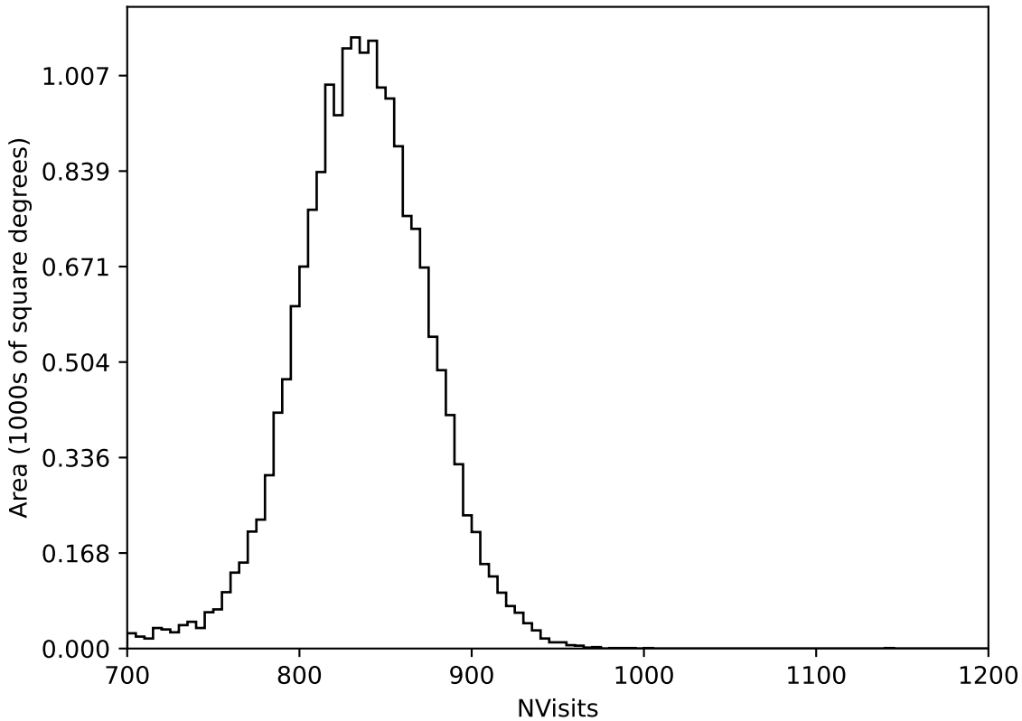
start_date_do-270v3.4_10yrs All sky all bands: NVisits
