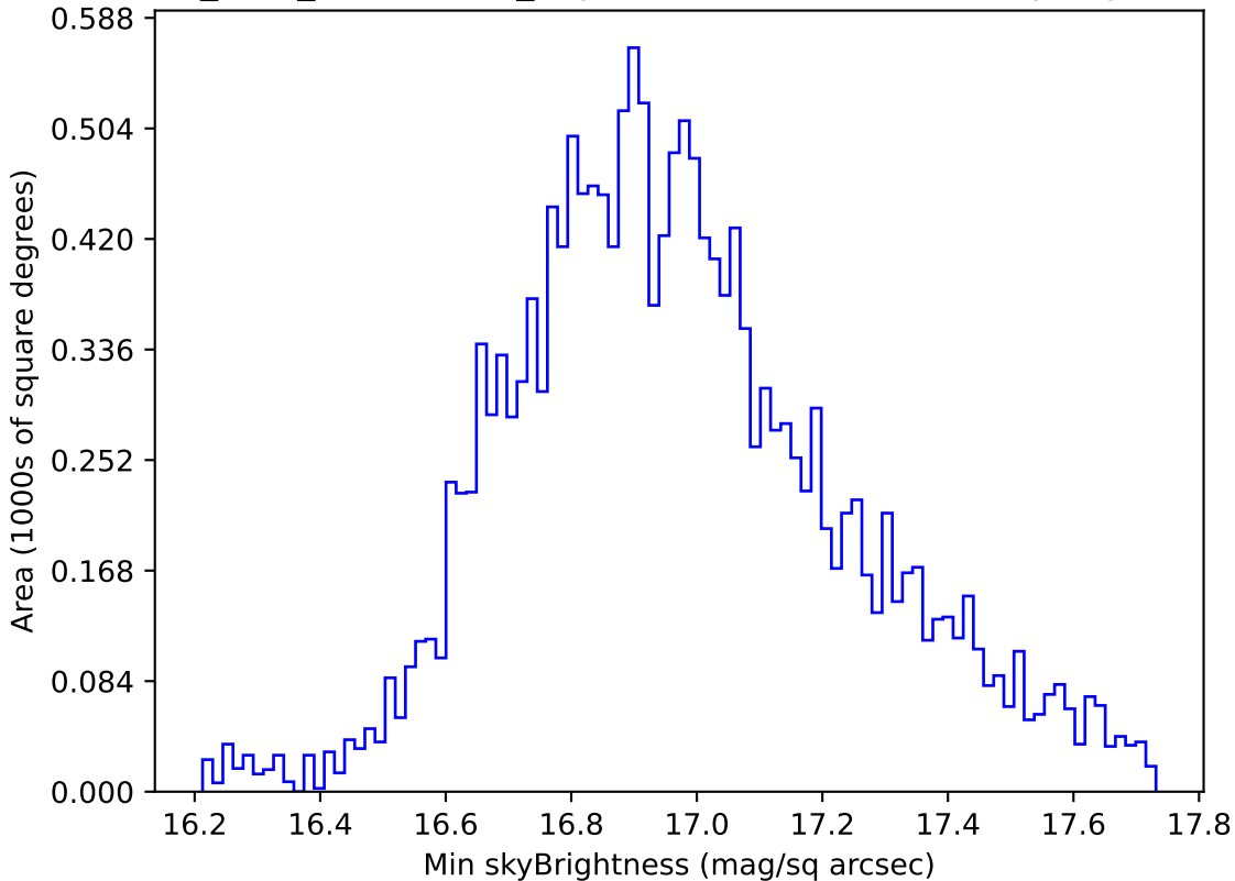
start_date_do-270v3.4_10yrs WFD all bands: Min skyBrightness
