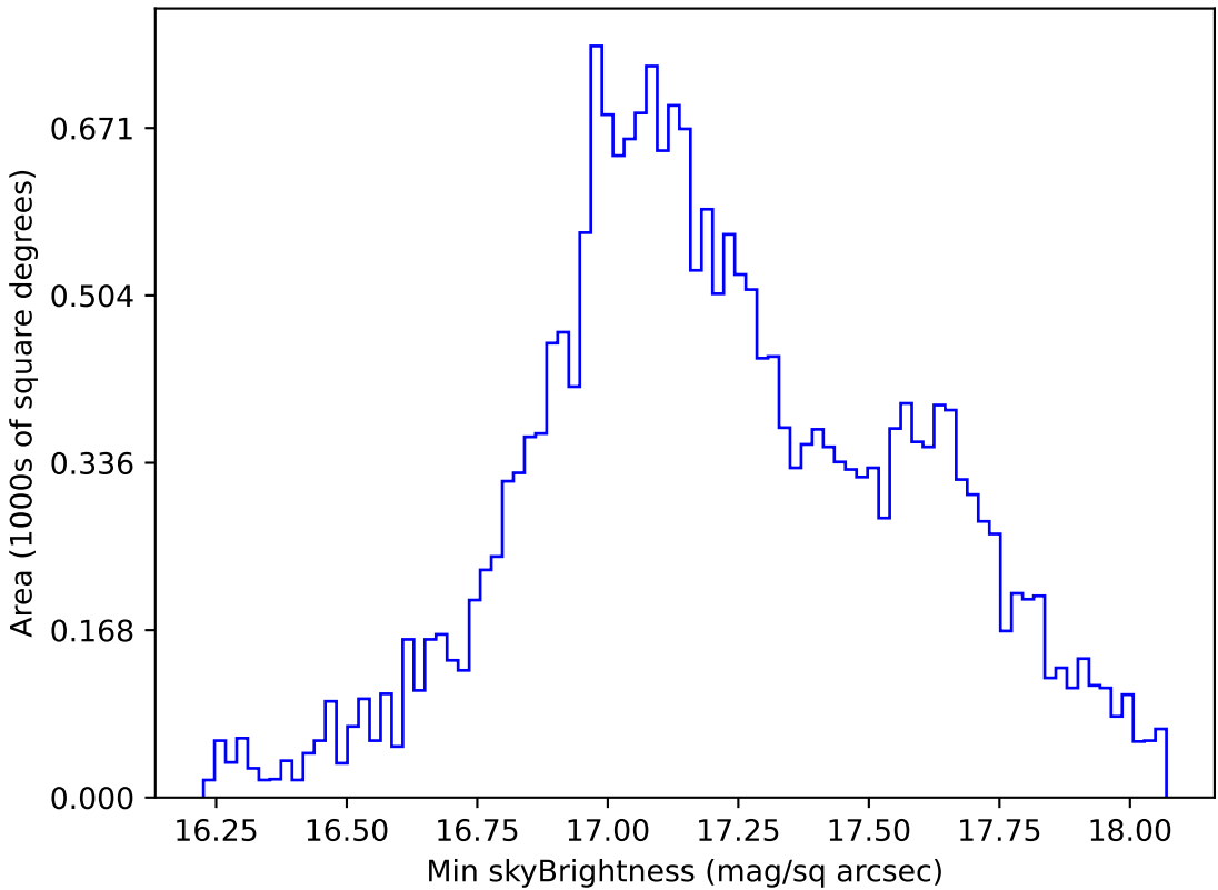
start_date_do-270v3.4_10yrs All sky y band: Min skyBrightness
