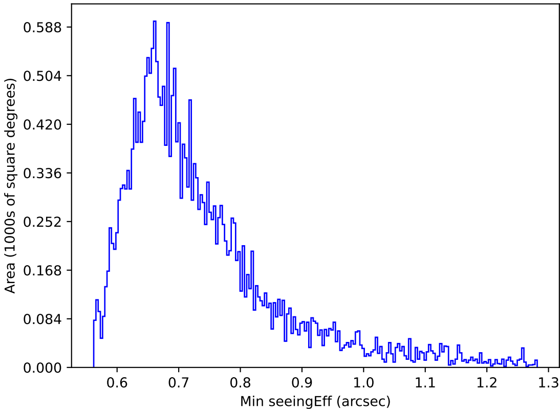
start_date_do-270v3.4_10yrs Yr 1 z band: Min seeingEff
