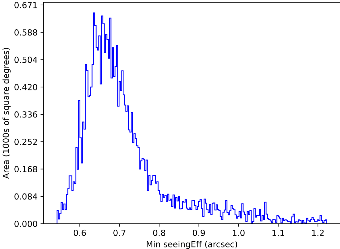
start_date_do-270v3.4_10yrs Yr 1 i band: Min seeingEff
