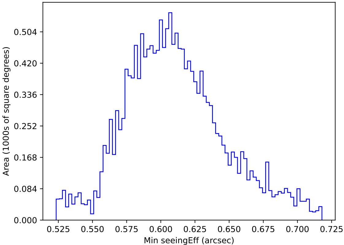
start_date_do-270v3.4_10yrs WFD i band: Min seeingEff
