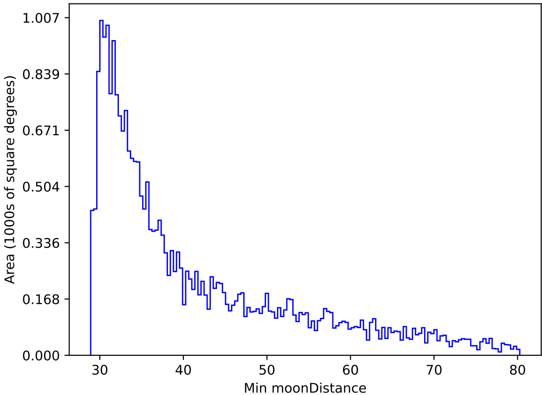
start_date_do-270v3.4_10yrs All sky r band: Min moonDistance
