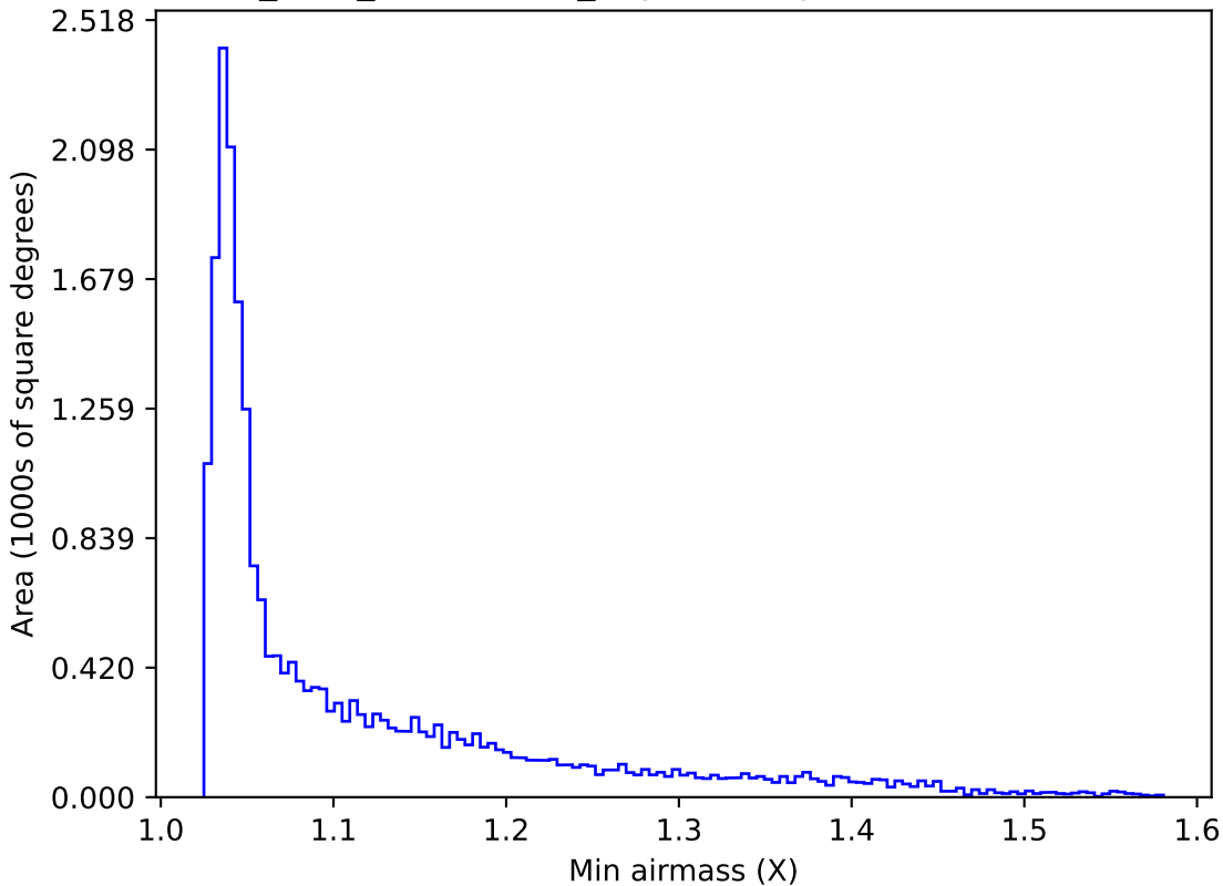
start_date_do-270v3.4_10yrs All sky u band: Min airmass
