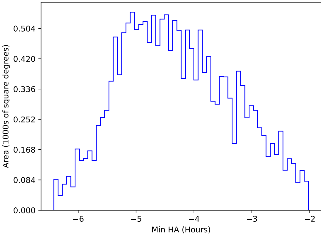
start_date_do-270v3.4_10yrs WFD i band: Min HA
