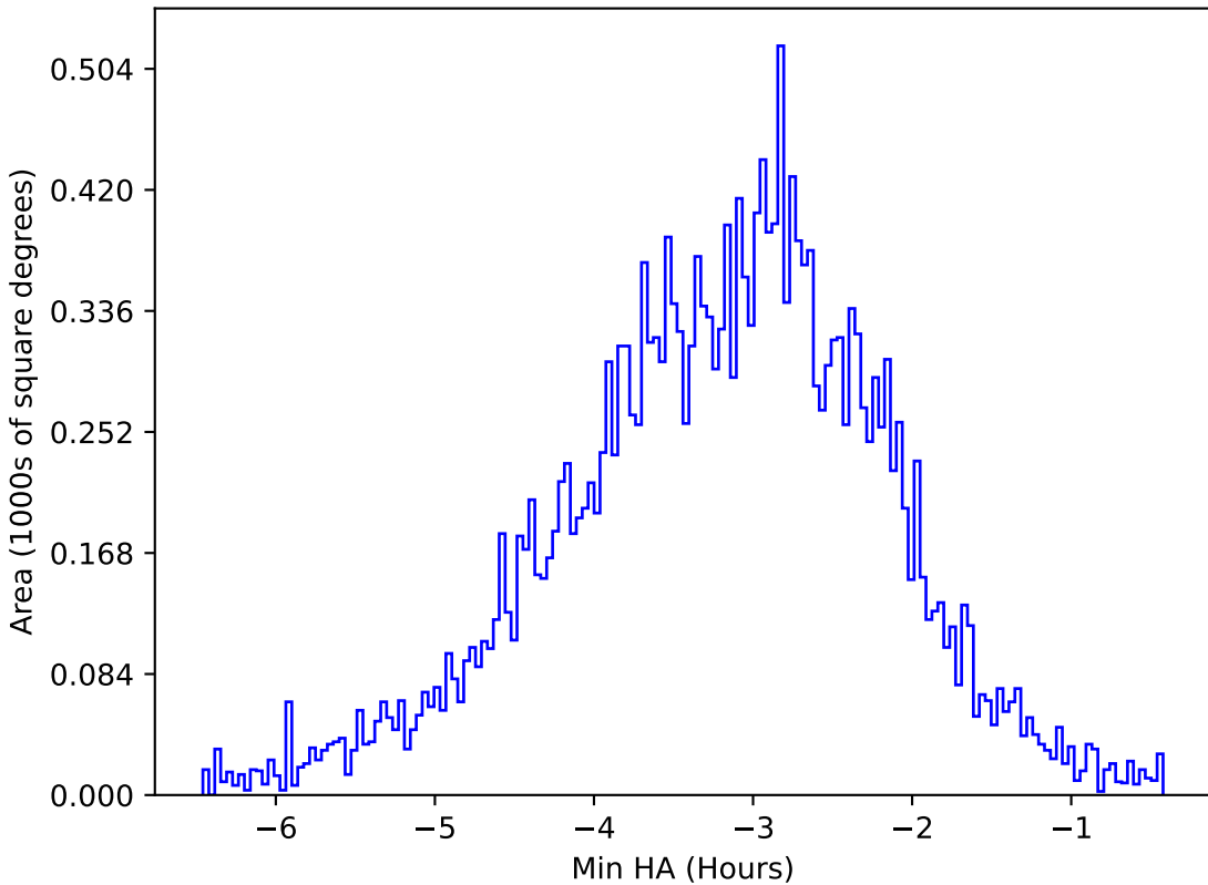
start_date_do-270v3.4_10yrs All sky u band: Min HA
