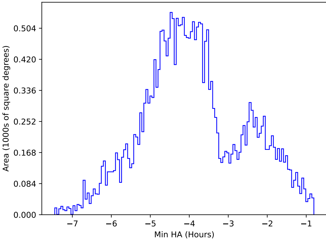
start_date_do-270v3.4_10yrs All sky g band: Min HA
