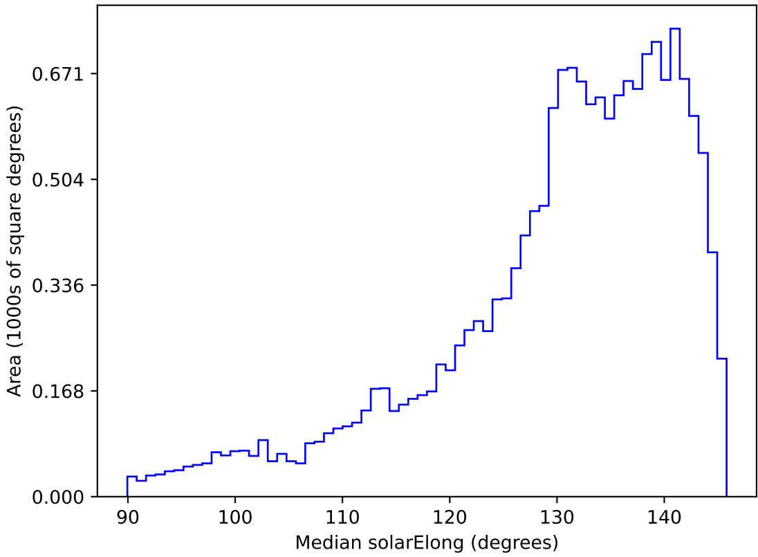
start_date_do-270v3.4_10yrs WFD all bands: Median solarElong
