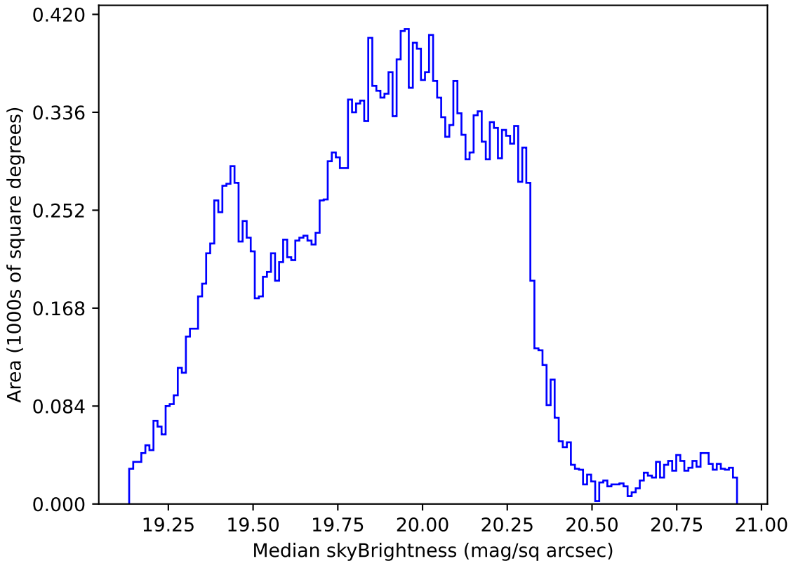
start_date_do-270v3.4_10yrs Yr 1 all bands: Median skyBrightness
