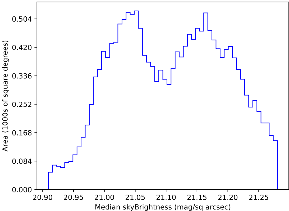
start_date_do-270v3.4_10yrs WFD r band: Median skyBrightness
