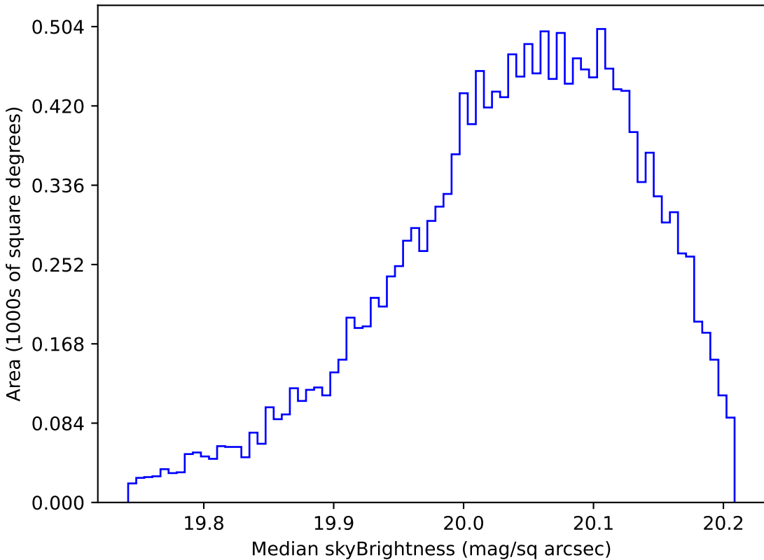
start_date_do-270v3.4_10yrs WFD i band: Median skyBrightness
