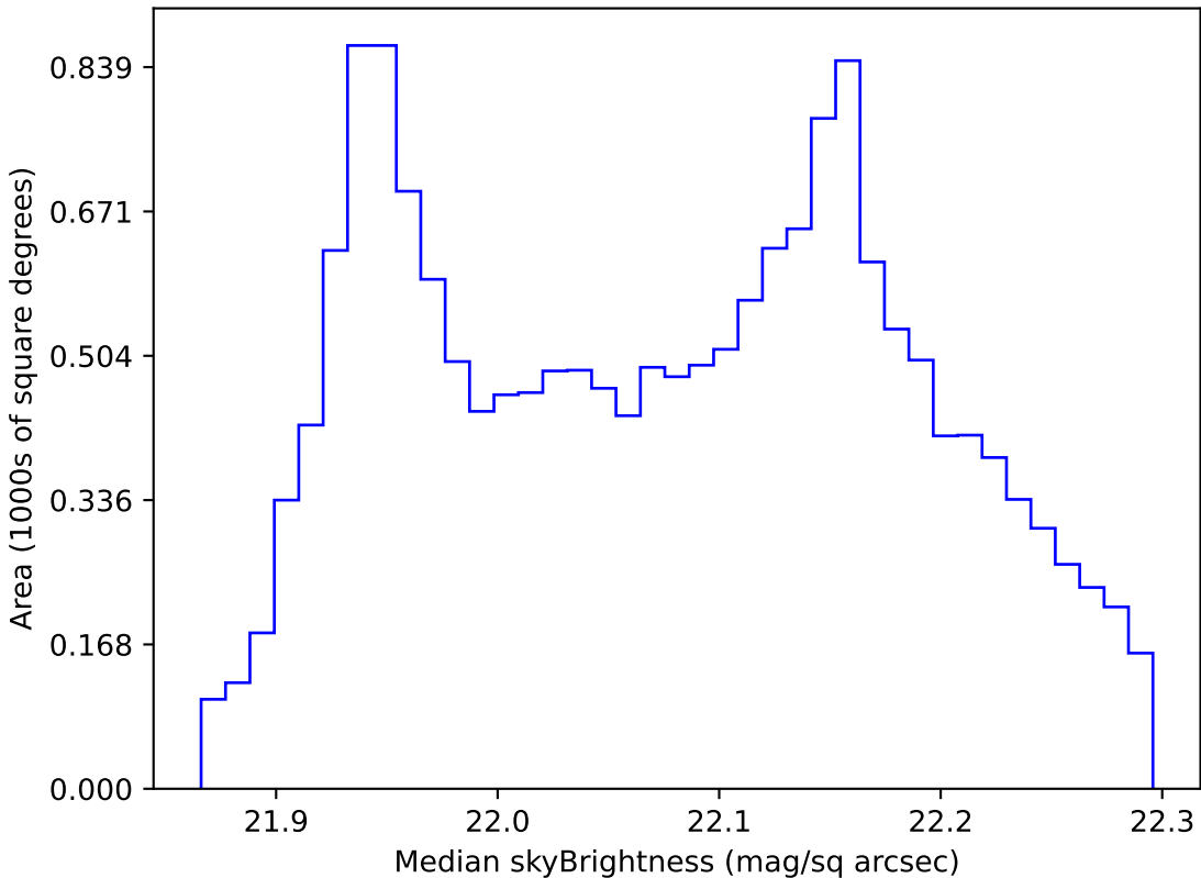
start_date_do-270v3.4_10yrs WFD g band: Median skyBrightness
