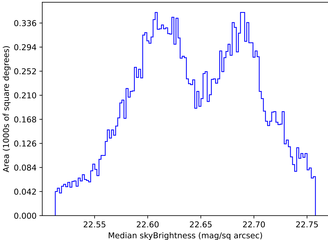
start_date_do-270v3.4_10yrs All sky u band: Median skyBrightness
