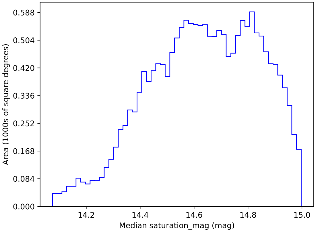
start_date_do-270v3.4_10yrs WFD r band: Median saturation_mag
