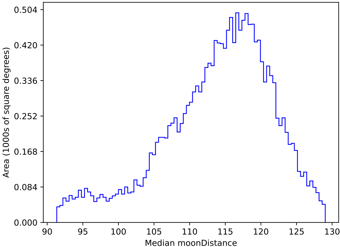
start_date_do-270v3.4_10yrs WFD r band: Median moonDistance
