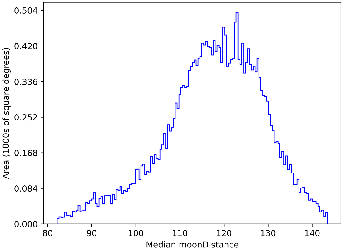
start_date_do-270v3.4_10yrs All sky g band: Median moonDistance
