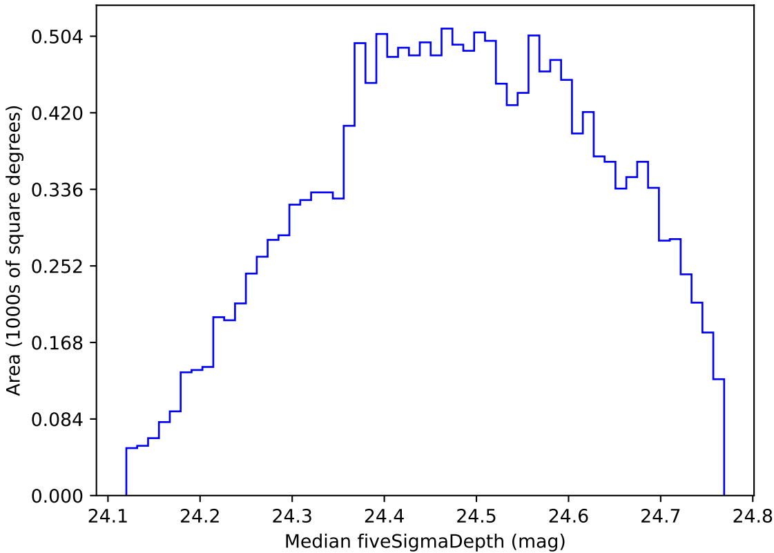
start_date_do-270v3.4_10yrs WFD g band: Median fiveSigmaDepth
