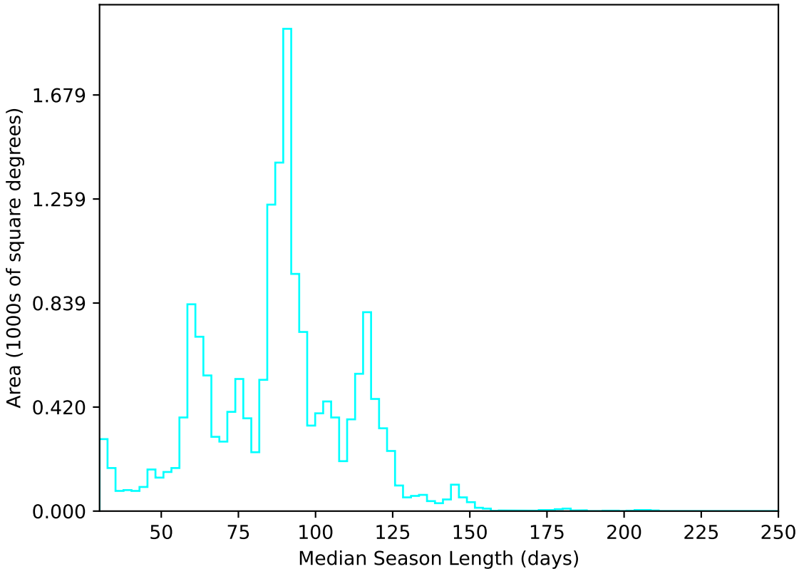
start_date_do-270v3.4_10yrs WFD u band: Median Season Length
