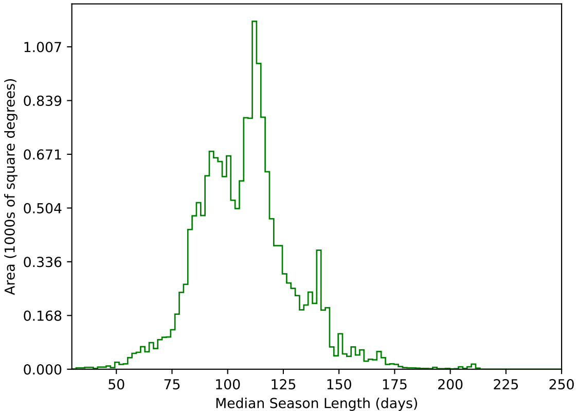
start_date_do-270v3.4_10yrs WFD g band: Median Season Length
