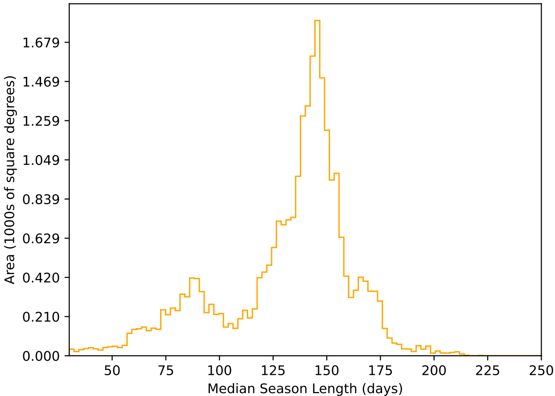
start_date_do-270v3.4_10yrs All sky r band: Median Season Length
