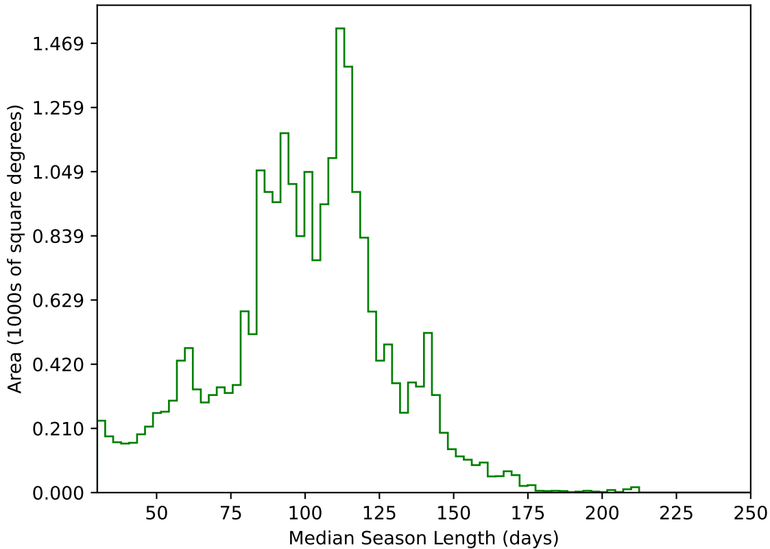
start_date_do-270v3.4_10yrs All sky g band: Median Season Length
