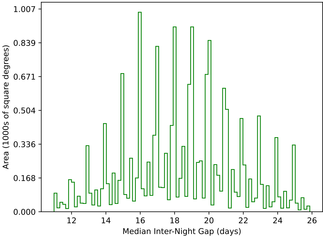
start_date_do-270v3.4_10yrs WFD g band: Median Inter-Night Gap
