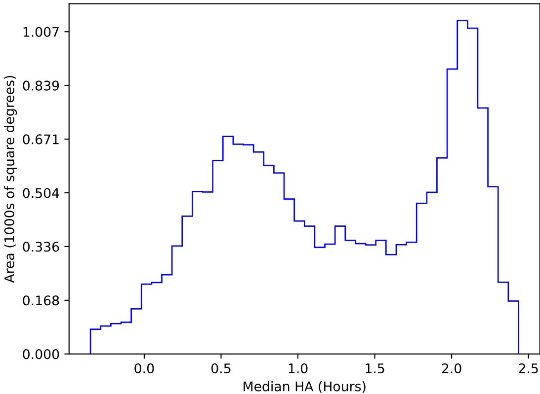
start_date_do-270v3.4_10yrs WFD y band: Median HA
