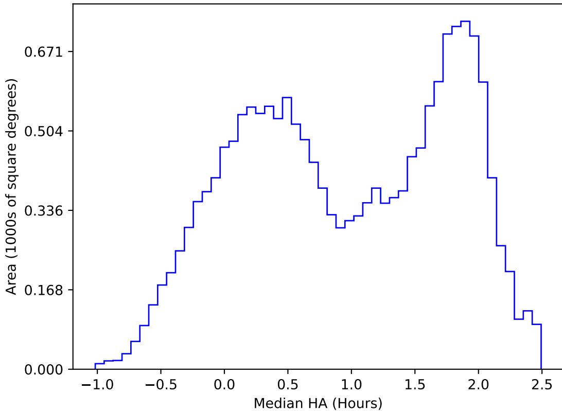
start_date_do-270v3.4_10yrs WFD u band: Median HA
