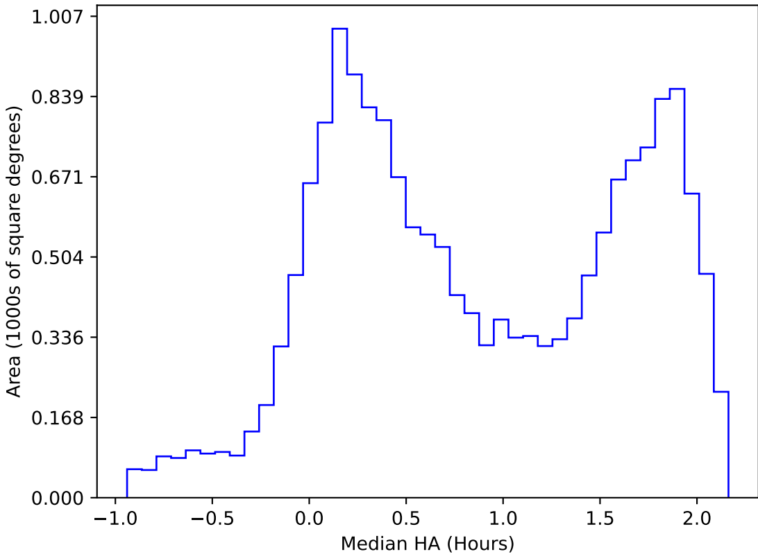
start_date_do-270v3.4_10yrs WFD r band: Median HA
