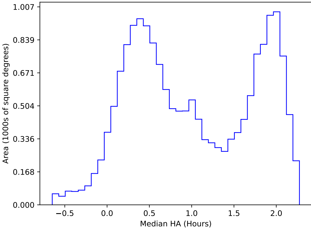
start_date_do-270v3.4_10yrs WFD i band: Median HA
