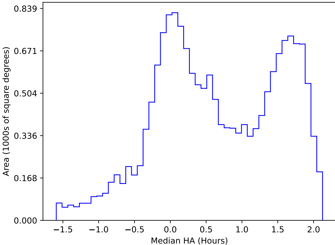
start_date_do-270v3.4_10yrs WFD g band: Median HA
