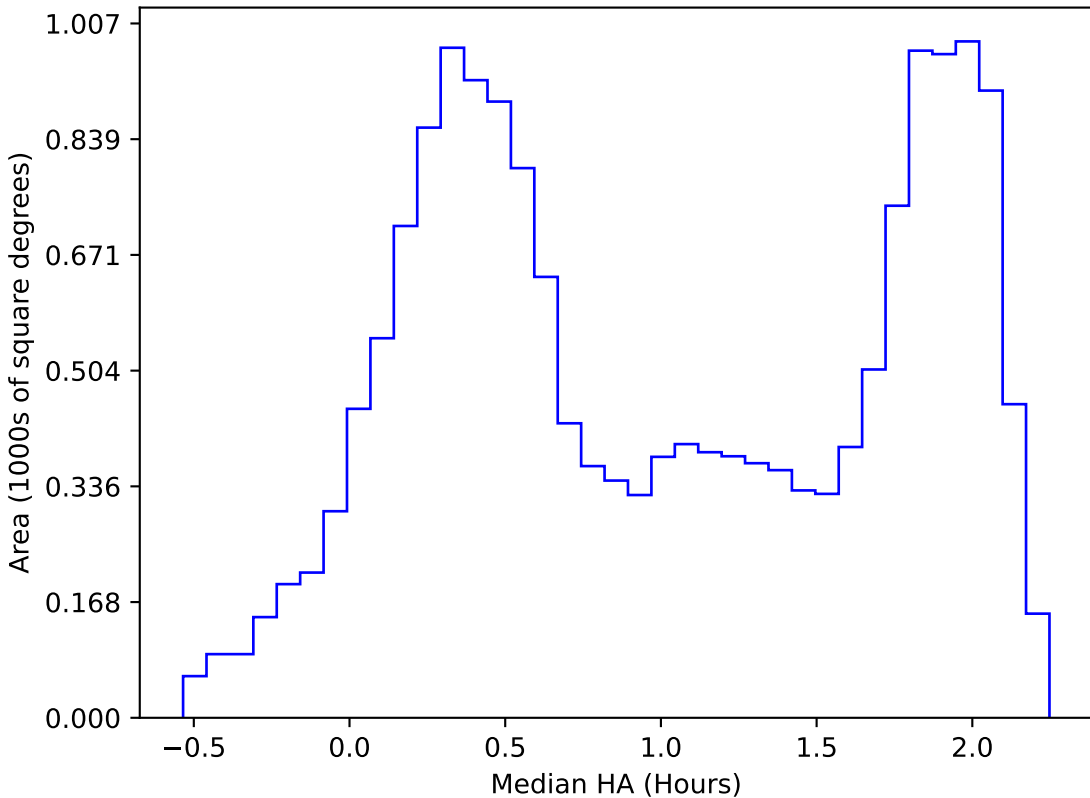
start_date_do-270v3.4_10yrs WFD all bands: Median HA
