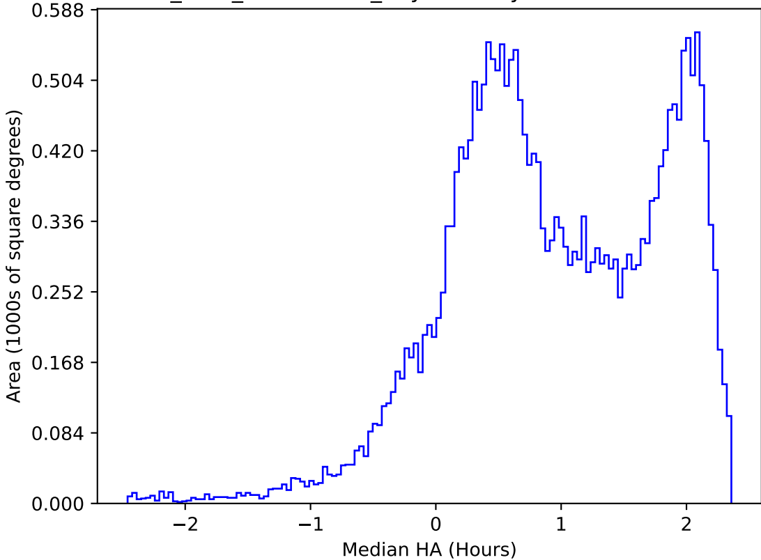
start_date_do-270v3.4_10yrs All sky z band: Median HA
