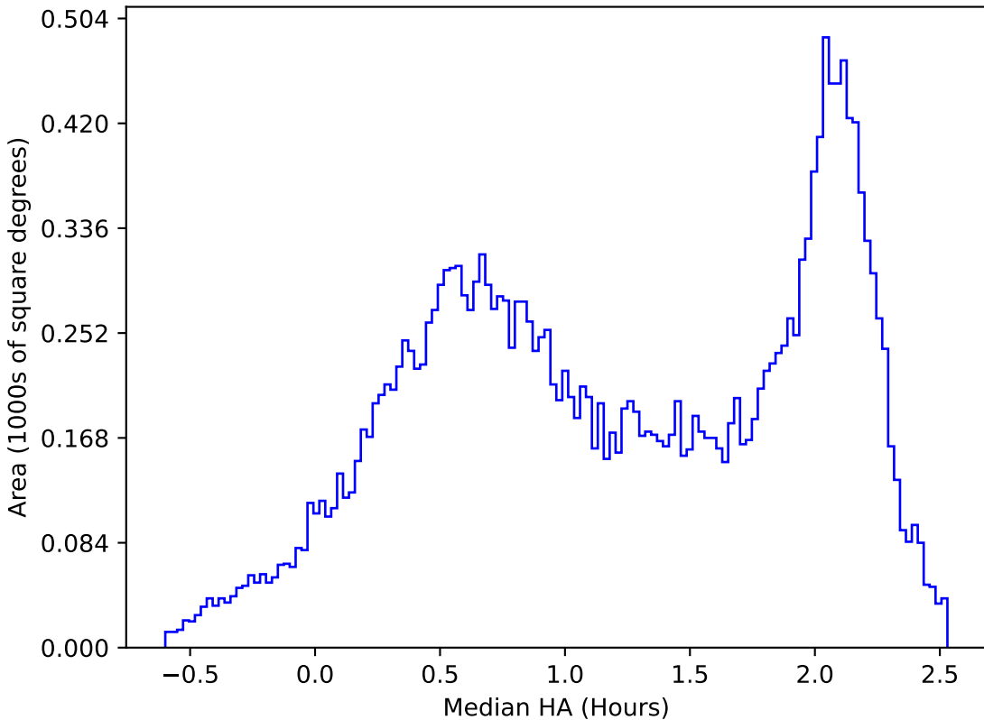
start_date_do-270v3.4_10yrs All sky y band: Median HA
