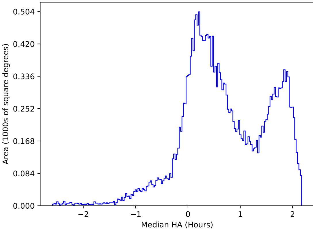
start_date_do-270v3.4_10yrs All sky r band: Median HA
