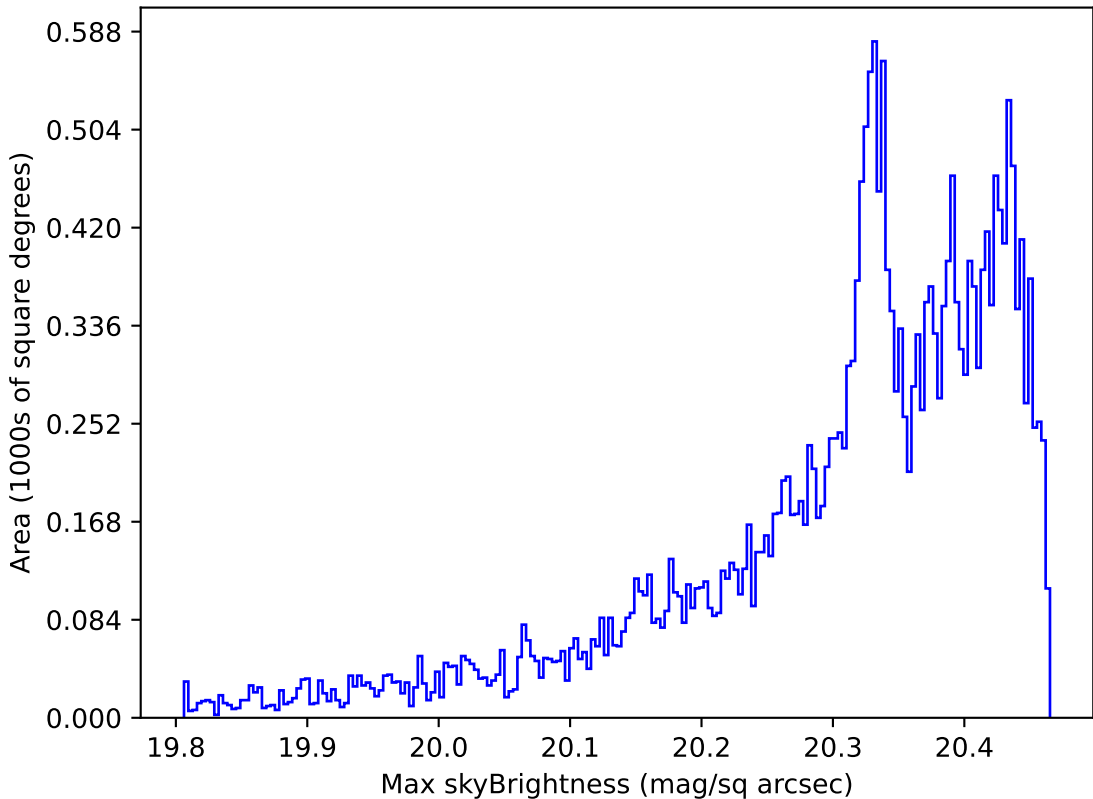
start_date_do-270v3.4_10yrs All sky i band: Max skyBrightness
