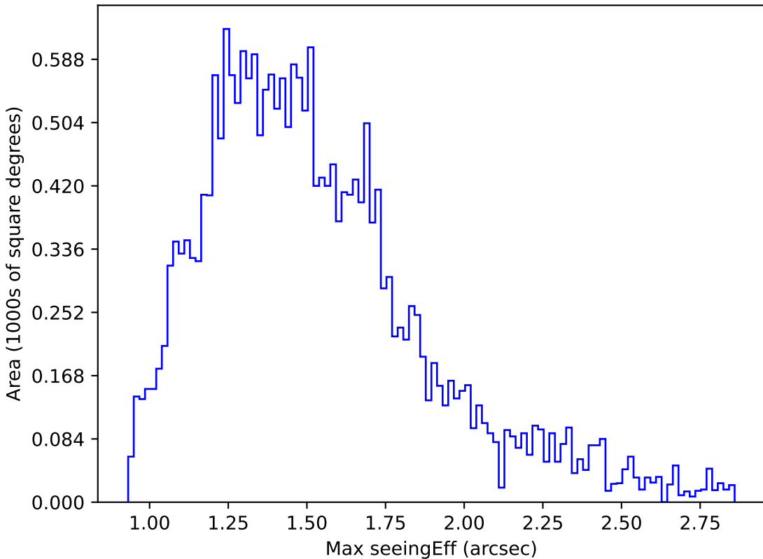
start_date_do-270v3.4_10yrs Yr 1 y band: Max seeingEff
