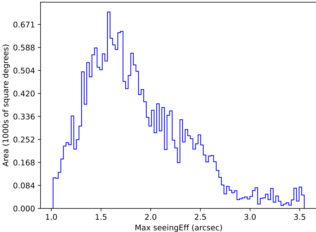
start_date_do-270v3.4_10yrs Yr 1 u band: Max seeingEff
