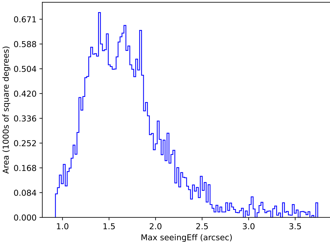
start_date_do-270v3.4_10yrs Yr 1 g band: Max seeingEff
