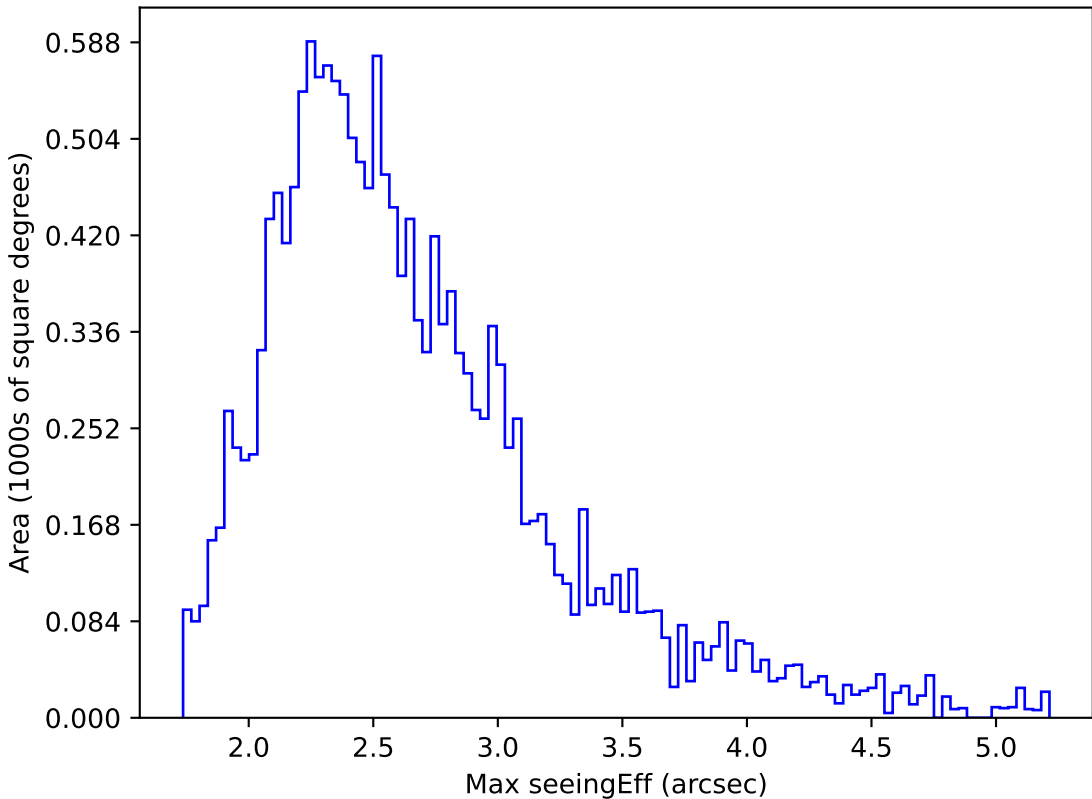
start_date_do-270v3.4_10yrs WFD i band: Max seeingEff
