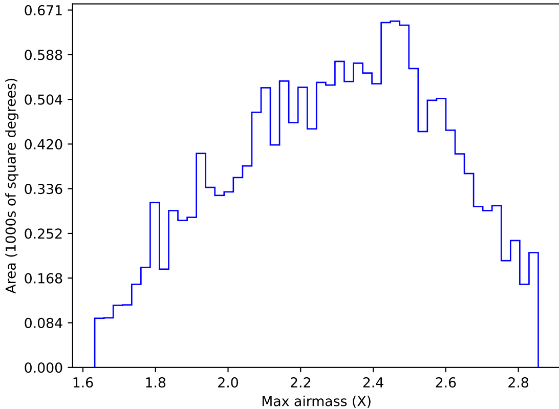
start_date_do-270v3.4_10yrs WFD y band: Max airmass
