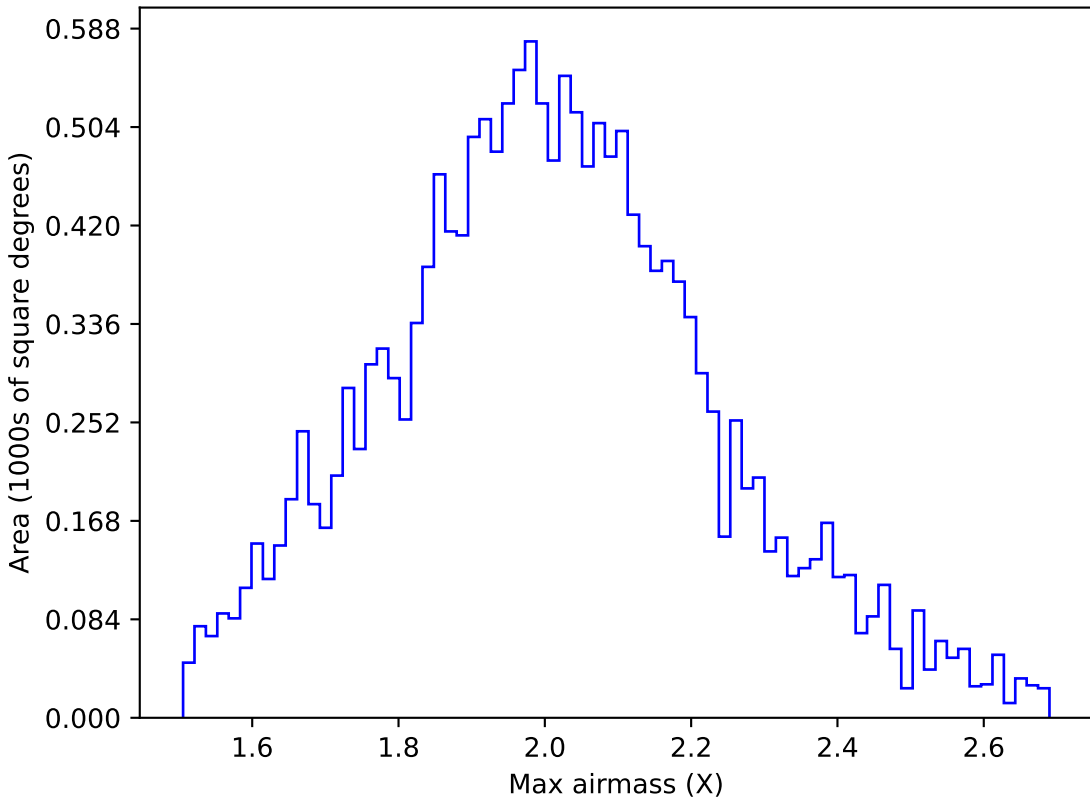
start_date_do-270v3.4_10yrs WFD g band: Max airmass
