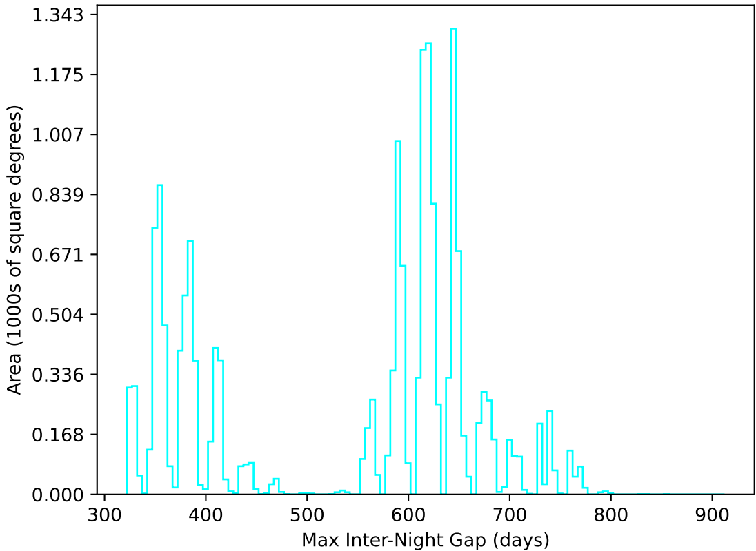
start_date_do-270v3.4_10yrs WFD u band: Max Inter-Night Gap
