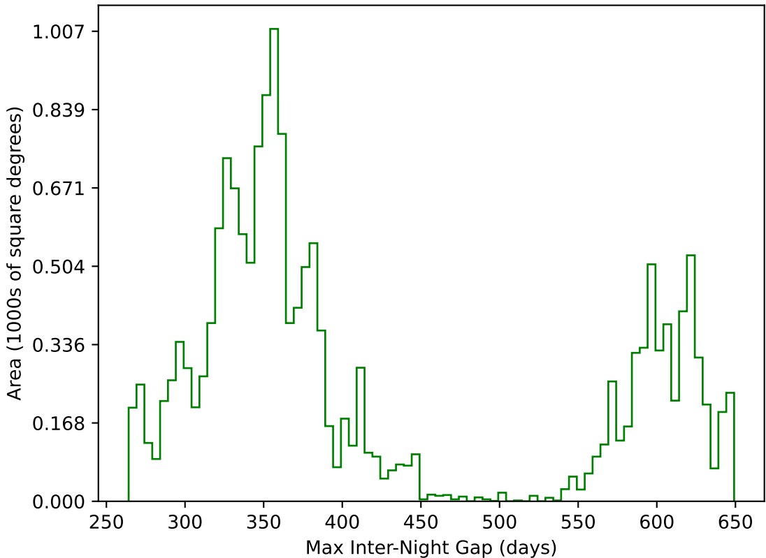
start_date_do-270v3.4_10yrs WFD g band: Max Inter-Night Gap
