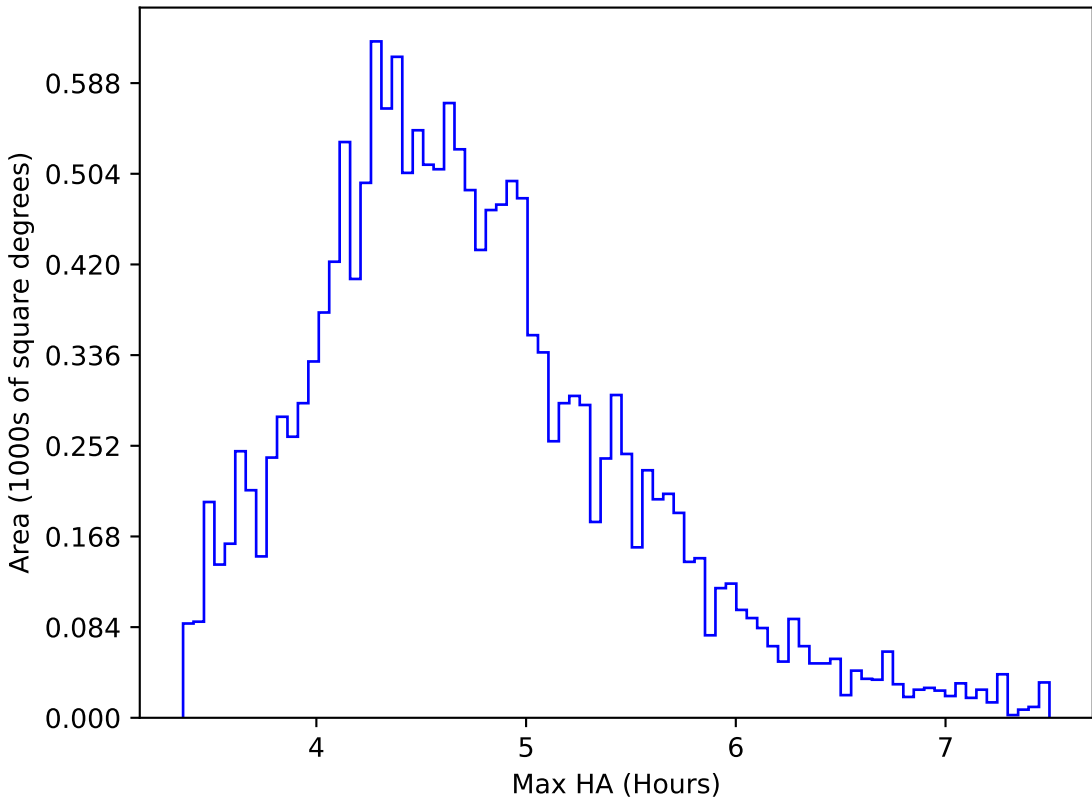
start_date_do-270v3.4_10yrs WFD y band: Max HA
