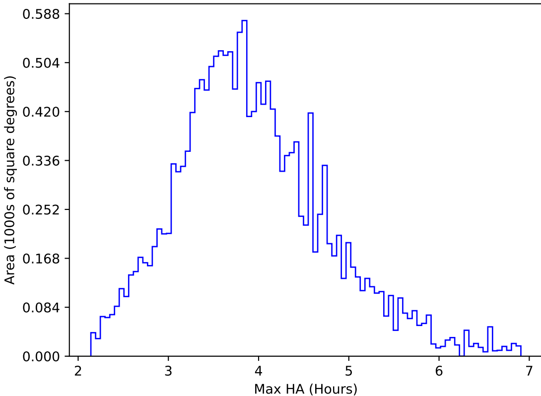
start_date_do-270v3.4_10yrs WFD g band: Max HA
