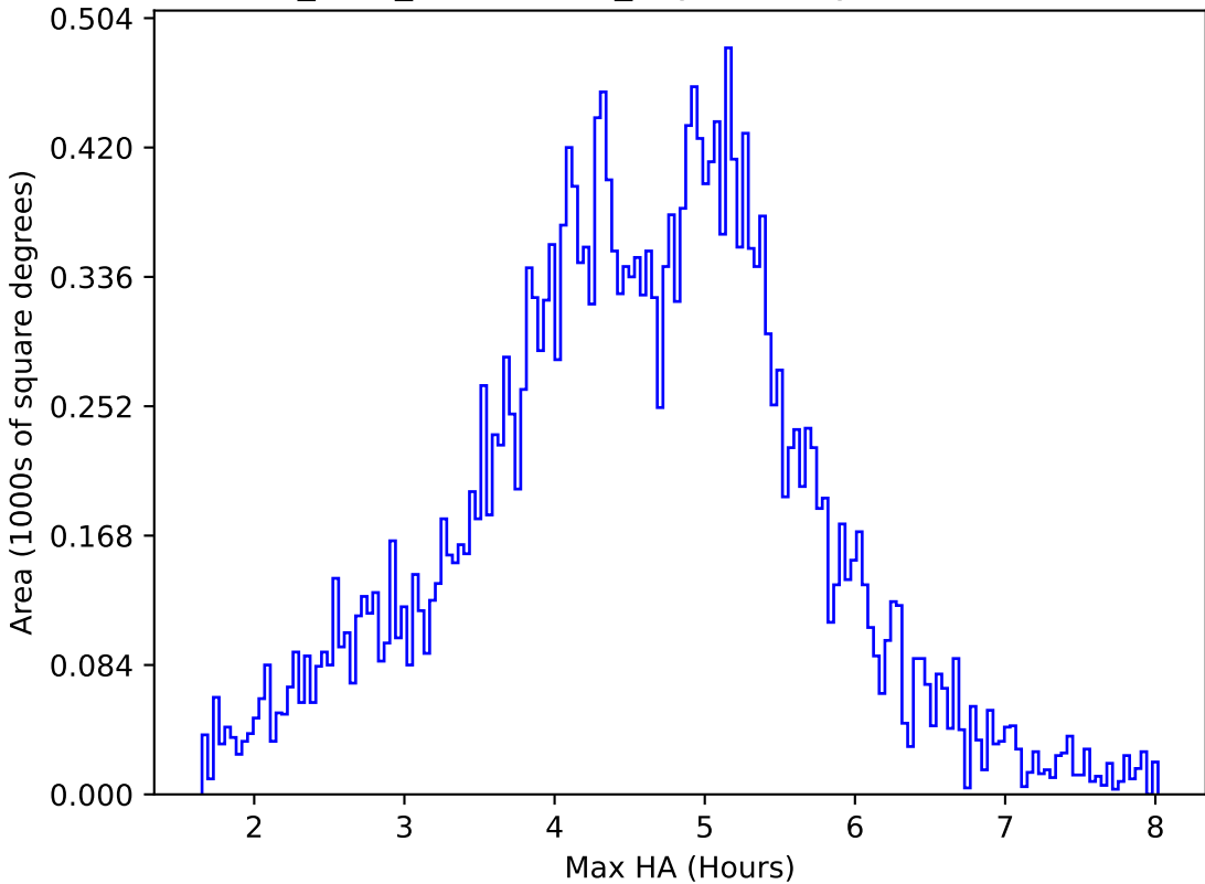
start_date_do-270v3.4_10yrs All sky z band: Max HA
