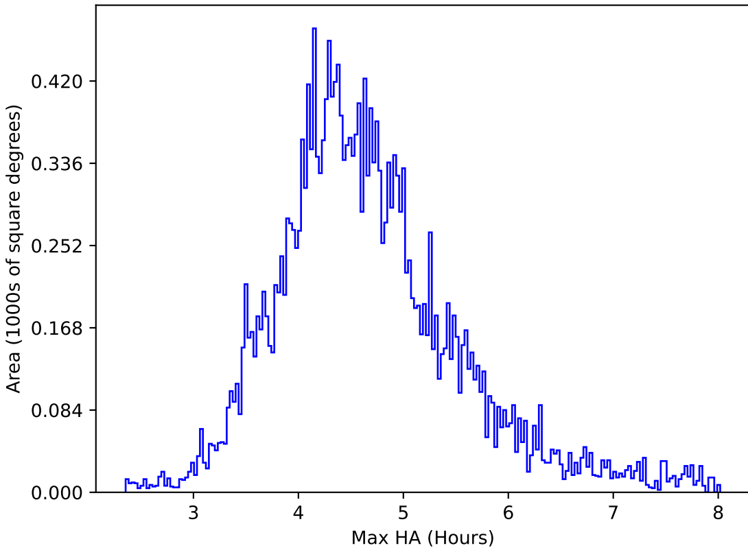
start_date_do-270v3.4_10yrs All sky y band: Max HA
