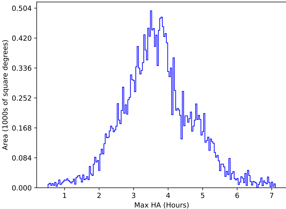
start_date_do-270v3.4_10yrs All sky u band: Max HA
